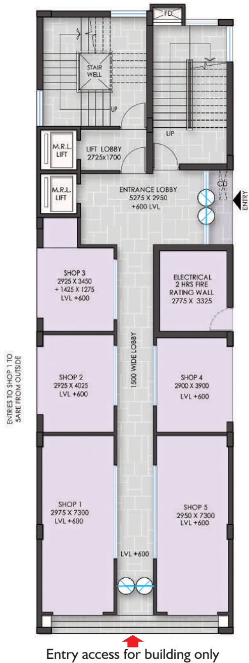
BLOCK 5 (GROUND FLOOR)
